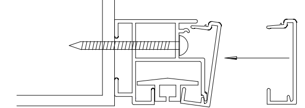
Flush Mount
