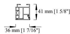
Guide Rail
