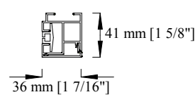
Guide Rail
